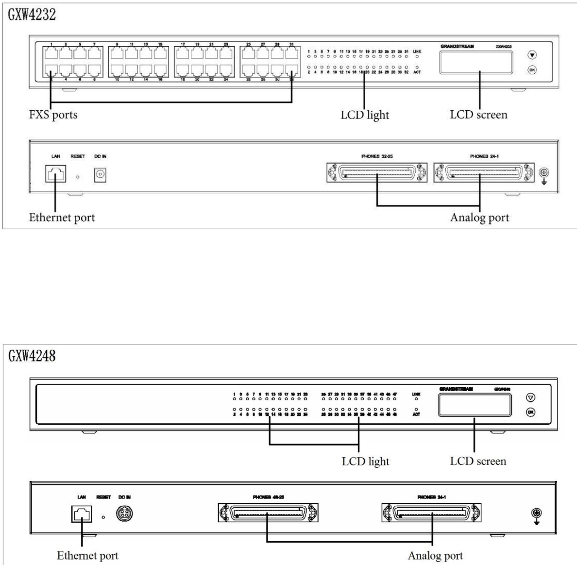
FIGURE 1: DIAGRAM OF GXW4216/24/32/48 PANEL
